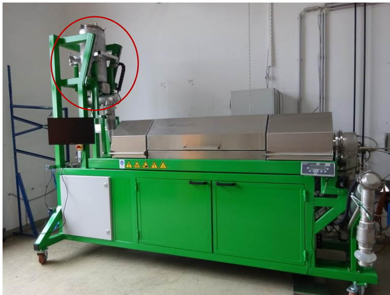
Figure 4: The used rotary kiln system, with the residue storage marked in red.
