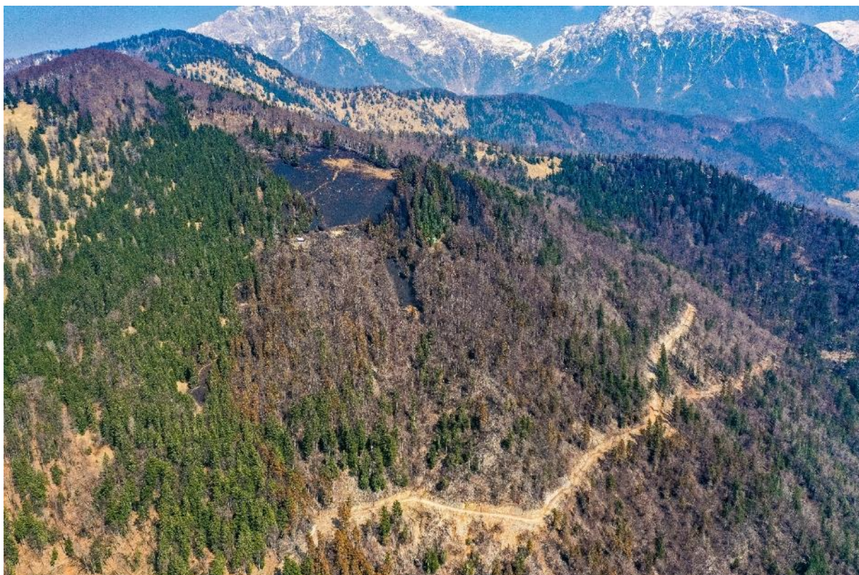
Figure 19: Post-fire landscape of Potoška Gora, year 2022, photo: Primož Šenk
