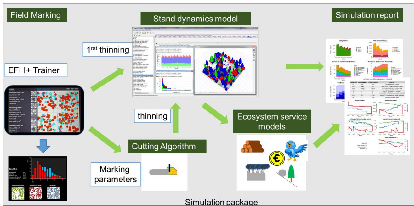
Figure 6: Principle of the R package connecting the I+Trainer field marking tool to the forest stand dynamics simulator Samsara
