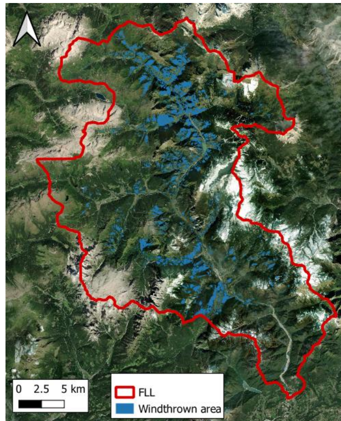
Figure 1: localization of the windthrown areas within the boundaries of the Alto Agordino forest living lab area.
