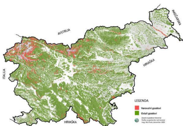
Figure 2: Protective forests of Slovenia (red colour)
