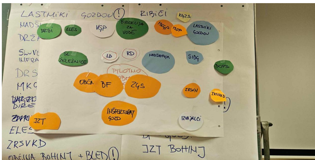
Figure 2: Venn diagram for stakeholder recognition and their relationship definition (example from FLL Soteska, Slovenia)
