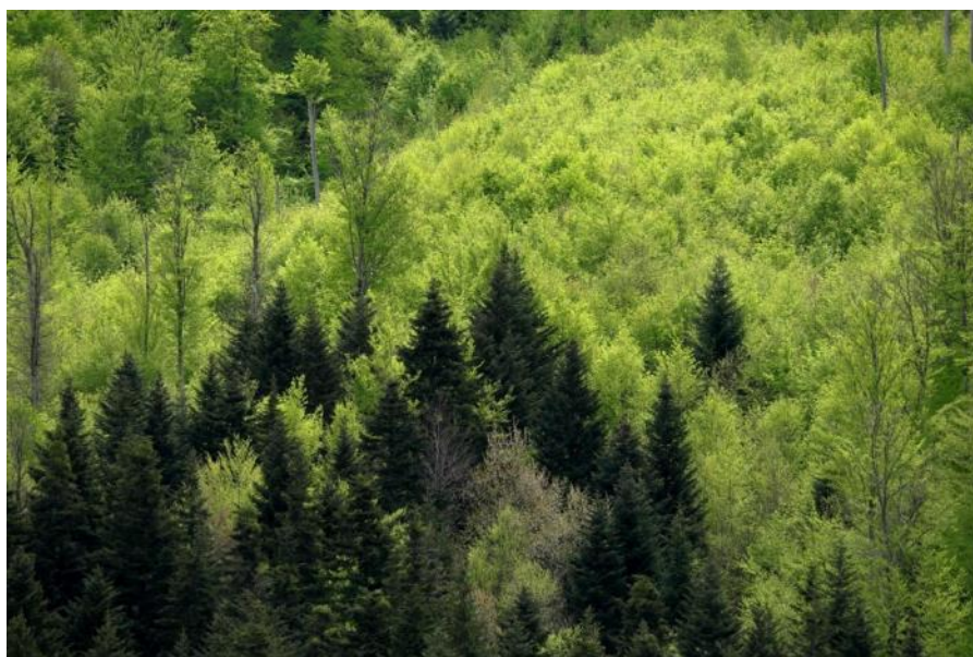
Figure 1: Natural regeneration after natural disturbance (photo: Slovenia Forest Service).
