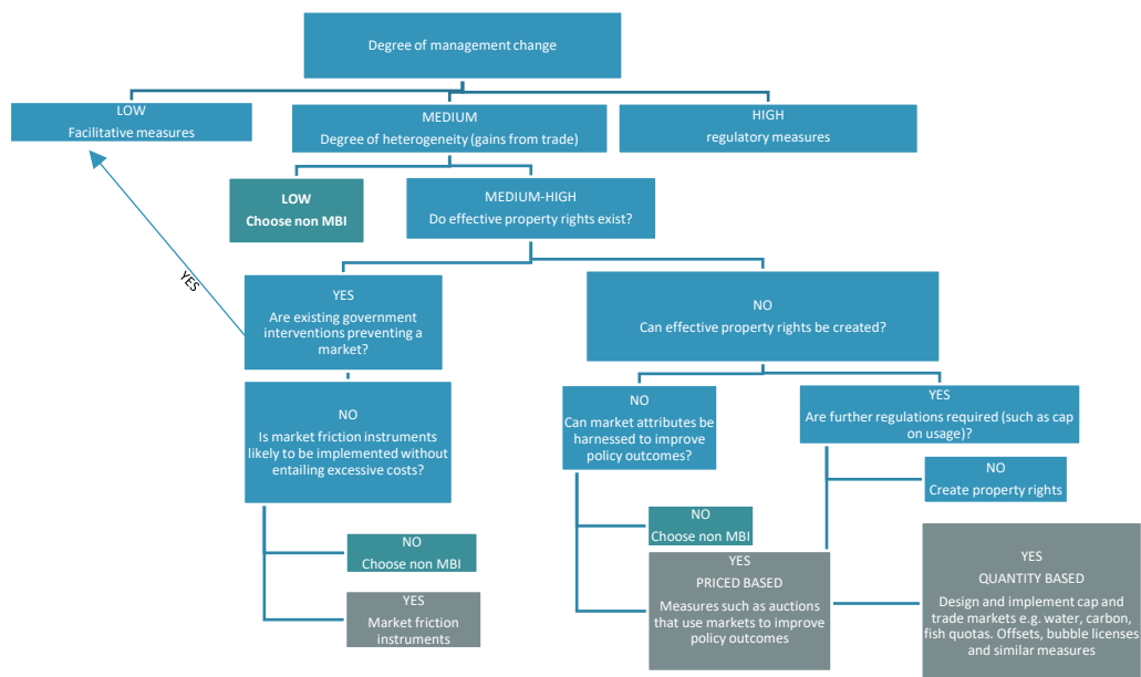
Figure 7. Decision tree for selecting appropriate MBIs
