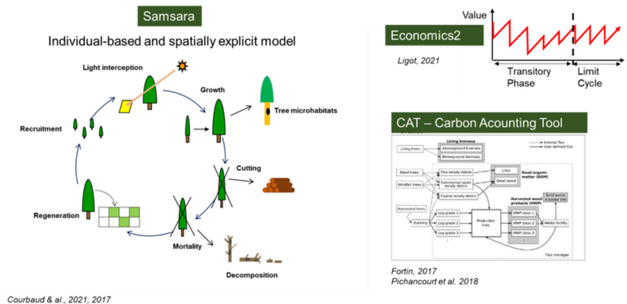
Figure 8: Principle of the Samsara model and of the associated libraries CAT and Economics2 in the software CAPSIS.
